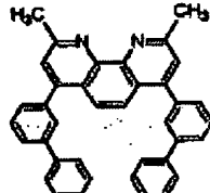
Structural formula 8:
